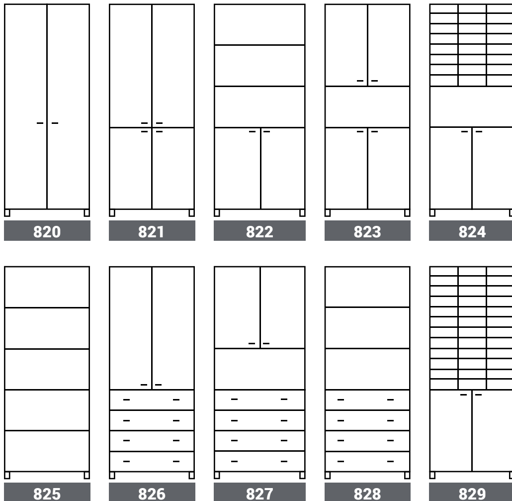
All units 2000 high x 800 wide x 400 deep
