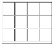
F - 1200L x 980H x 300D
